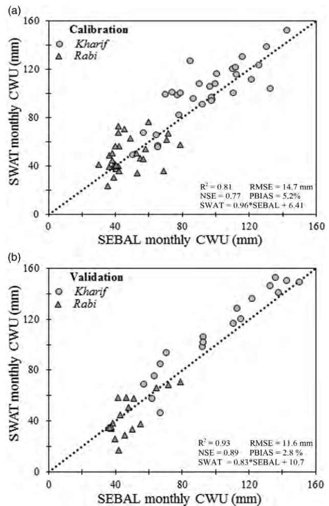
Figure 3 | Statistical comparison between SWAT and SEBAL estimated monthly CWU for the Rabi (Oct–Mar) and Kharif (Apr–Sep) seasons during (a) calibration (2005–2009) and (b) validation (2010–2012) periods.
