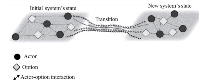
Figure 4. The conceptualisation of transition [22]
