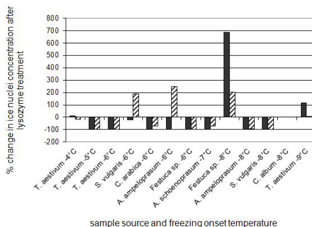
Fig. 4. Effect of lysozyme treatment on the abundance of ice nuclei in spore suspensions. The effect is presented as the percent of change in the number of ice nuclei per \text{mL} of spore suspension at the freezing onset temperature (black bars) and at one degree below the freezing onset temperature (hatched bars) for each sample. There was 0 % change in freezing behavior for spores from C. album for both temperatures.
