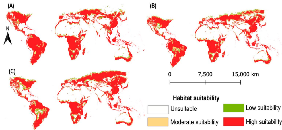
FIGURE 6 | Potential distribution of RPW under (A) current climatic conditions, (B) future climatic conditions projected under the SSP2–4.5 scenario, and (C) future climatic conditions projected under the SSP5–8.5 scenario. Predictions were generated using a risk index calculated from temperature-dependent development models for RPW.
