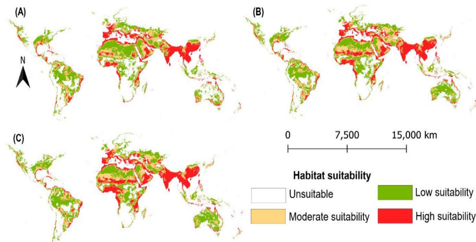
FIGURE 5 | Potential distribution of the red palm weevil (RPW) under (A) current climatic conditions, (B) future climatic conditions projected under the SSP2-4.5 scenario, and (C) future climatic conditions projected under the SSP5-8.5 scenario. Predictions were generated using an ensemble model integrating six machine-learning algorithms: Support vector machines (SVM), generalized additive model (GAM), generalized linear model (GLM), multivariate adaptive regression splines (MARS), boosted regression tree (BRT) and classification and regression tree (CART).
