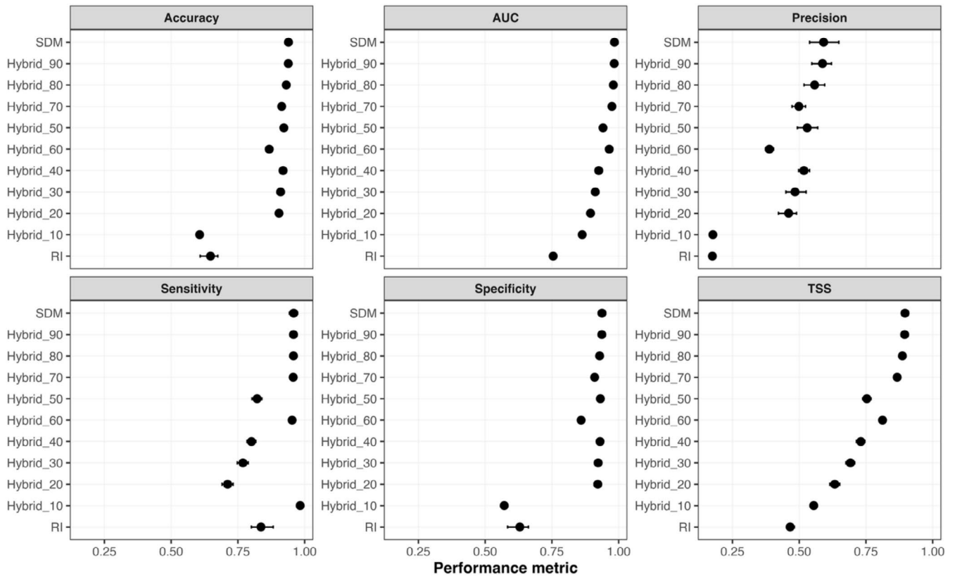
FIGURE 7 | Best-performing additive hybrid model identified through iterative weighting of mechanistic (phenology-based RI) and correlative (SDM) components.
