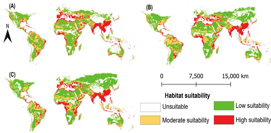
FIGURE 8 | Potential distribution of RPW under (A) current climatic conditions, (B) future climatic conditions projected under the SSP2-4.5 scenario, and (C) future climatic conditions projected under the SSP5-8.5 scenario. Predictions were generated using a combination of the ensemble ecological niche model and the temperature-dependent risk index.
