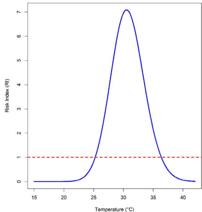
FIGURE 3 | Computed risk index of RPW under temperature range using ordinary differential equations.
