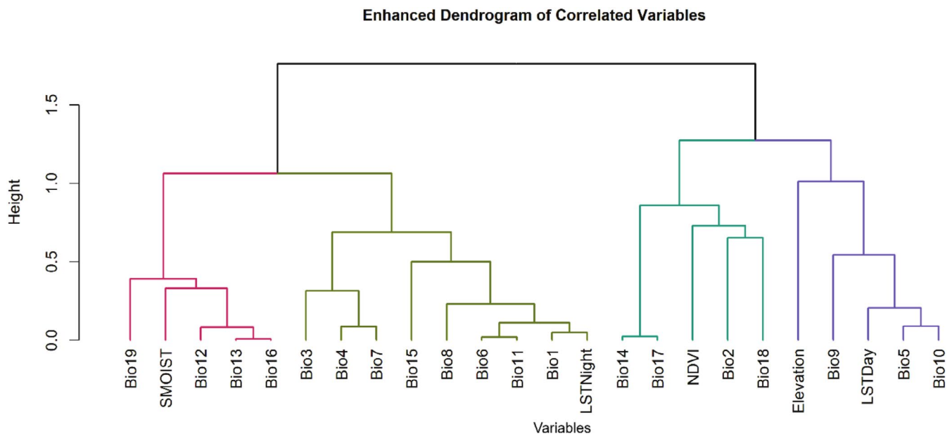
FIGURE 2 | The enhanced correlation distance dendrogram among the predictor variables. The height of the branch point indicates the level of similarity between clusters, with shorter branch points indicating higher similarity between the variables (stronger correlation between the variables).
