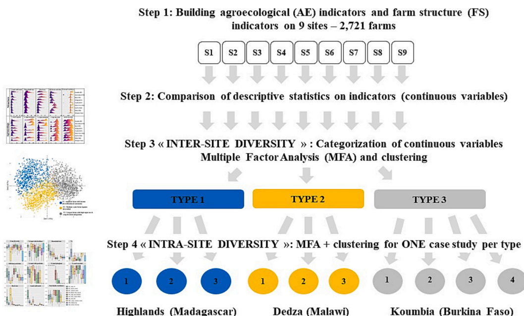
Fig. 3. Methodological diagram.
