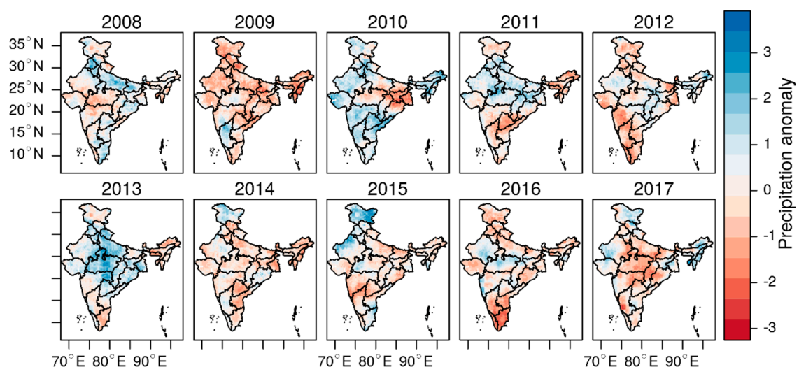
Figure 5. Spatio-temporal variation of precipitation anomalies in India, derived from TRMM 3B43 data for the period 2008 to 2017 based on the long term average and standard deviation of 2000 to 2017.
