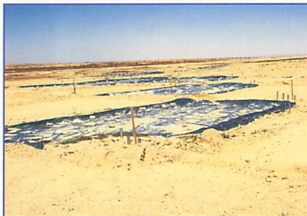
Plastic sheets ensures very high runoff coefficient; it is however, costly and mostly used for harvesting water to cash crops.
