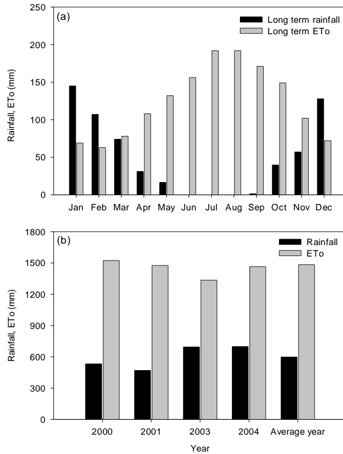
Figure 1. Monthly long term (1954-2010) rainfall and reference evapotranspiration (ET 0 )–(a) and annual rainfall and ET 0 during the four growing seasons (2000, 2001, 2003 and 2004) and during an average year (b).
