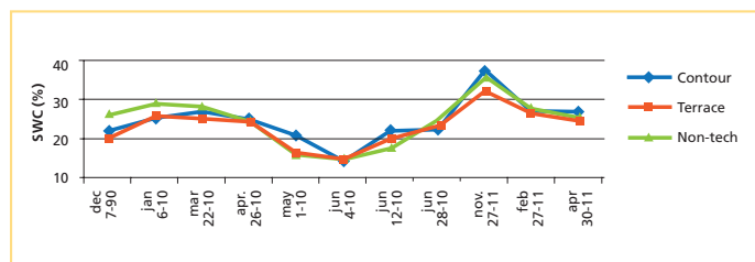
Soil water content (SWC) under contour ploughing and terracing compared to the control situation without technologies (non-tech).
