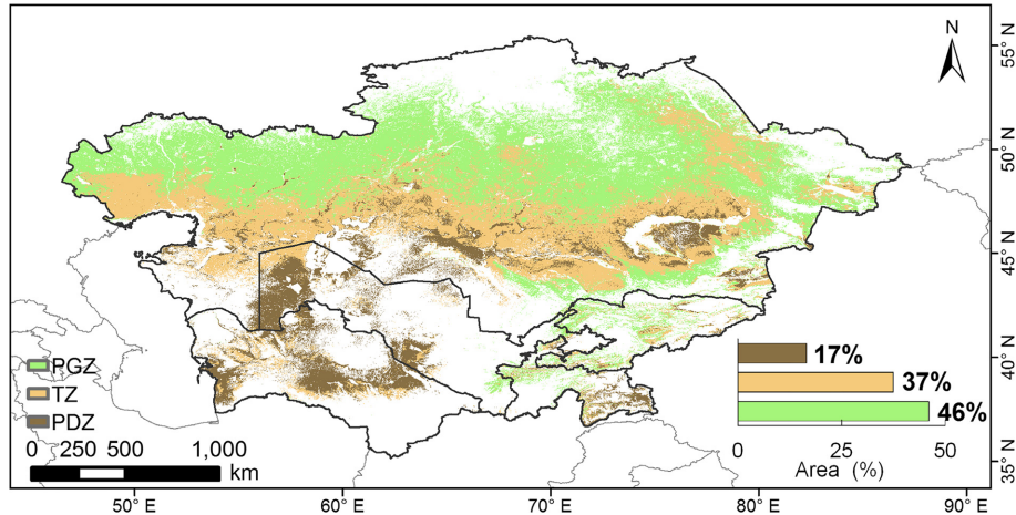
FIG. 5. Spatial distribution of persistent grassland zone (PGZ), transition zone (TZ), and persistent desert zone (PDZ). The inset shows the area percentages of different zones. The result data is available from https://doi.org/10.5061/dryad.12bd9 .
