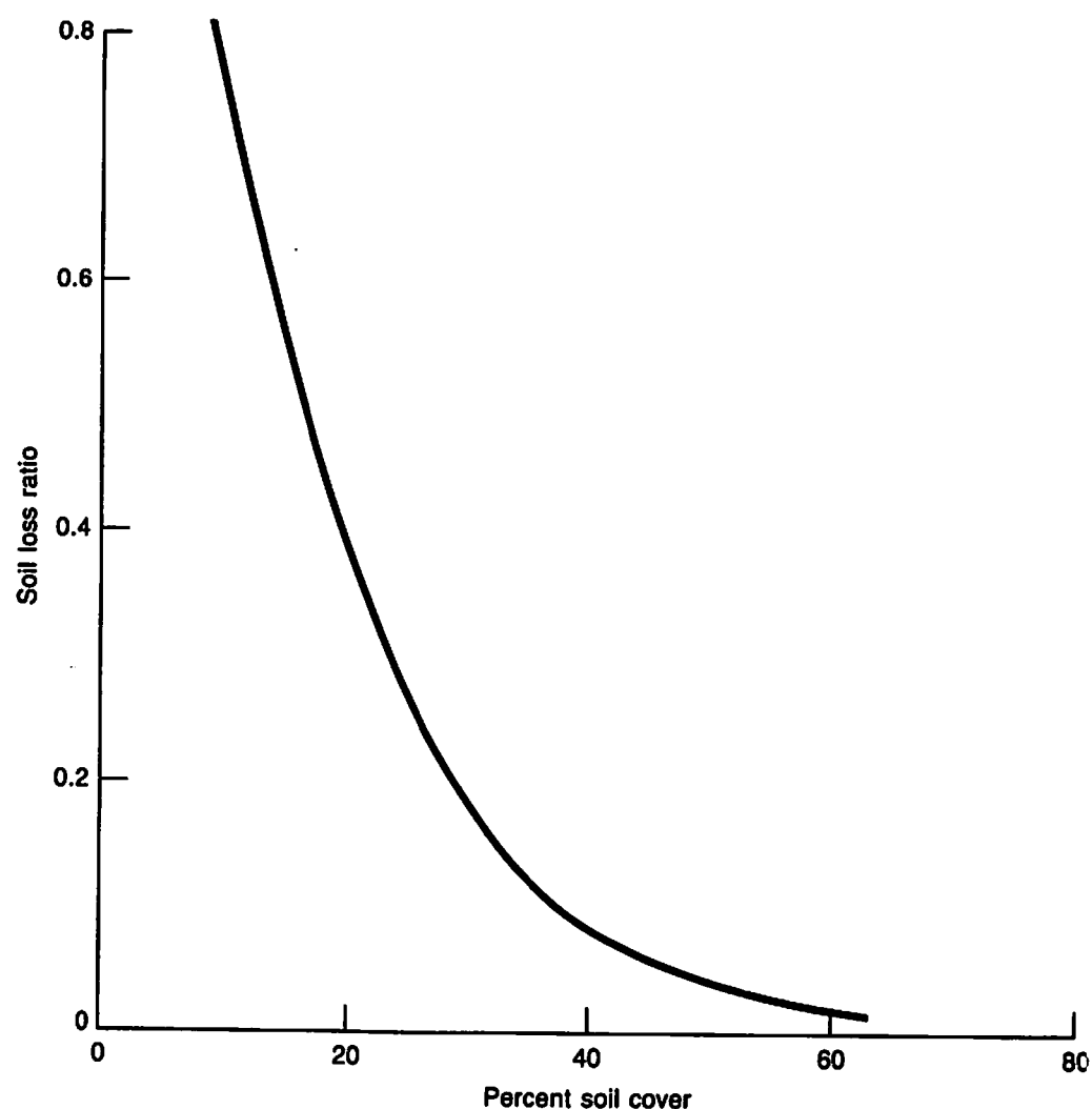
Figure 2. Relation between Soil Loss Ratio and Percent Soil Cover (Soil Loss with No Cover Equal to 1), when Various Percentages of Soil Surface Are Covered with Flat Nonerodible Material (Fryrear, 1985).
