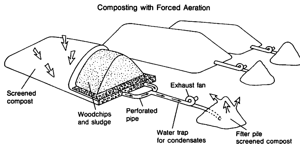
Figure 2. A Schematic Diagram of the Beltsville Aerated Rapid Composting Method for Composting Sewage Sludge and Other Organic Wastes.
