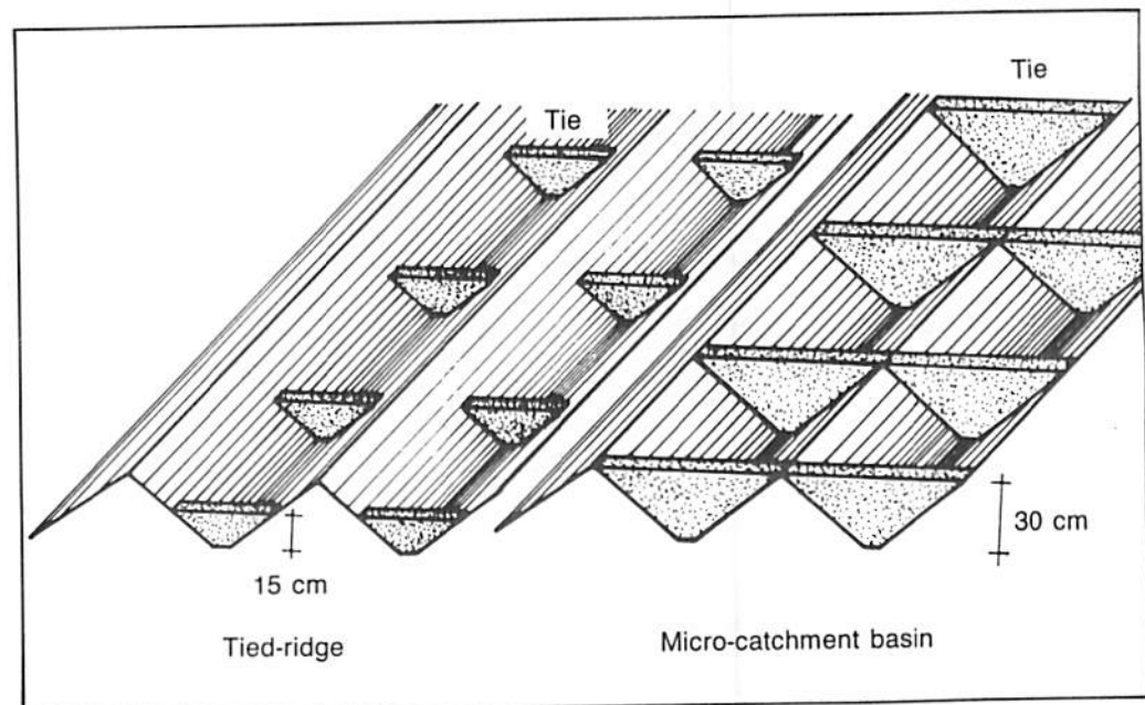
Figure 6. Schematic Diagram Showing the Cross Sections of Tied-Ridges and Micro-Catchment Basins.
