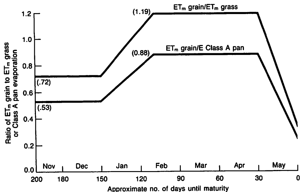
Figure 6. Curves for Use in Estimation of Water Requirements ( ET_m ) of Wheat and Barley in Mediterranean Zones. Based on Unpublished Lysimeter Studies by W.O. Pruitt and J.L. Hatfield on Barley (1969/70 and 1977/78) and Wheat (1976/77 and 1977/78) at University of California at Davis.
