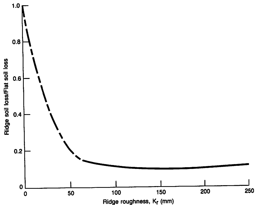
Figure 3. Relation between Soil Loss Ratio and Soil Ridge Roughness K_r with Wind Direction Normal to Ridges in the Wind Tunnel;
