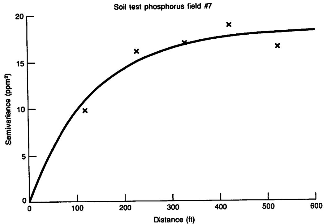
Figure 3. Semivariance Values and Exponential Semivariogram Model for 40 Soil Test Phosphorus Values on a Commercial Farm in the Columbia Basin of Washington.
