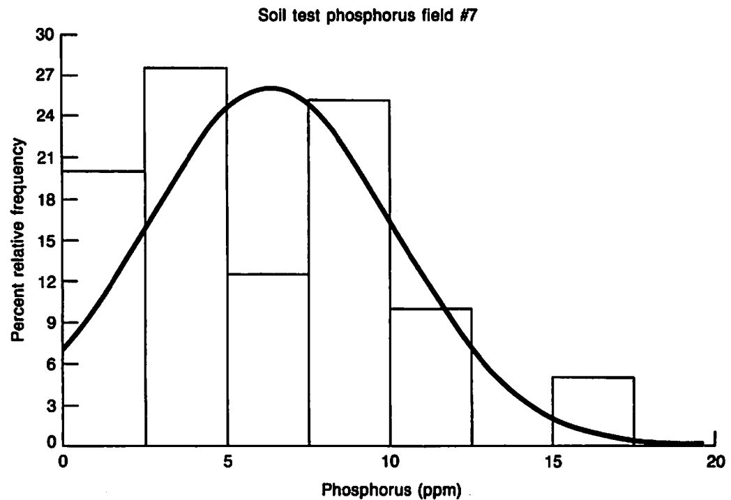
Figure 2. Frequency Distribution Diagram of Soil Test Phosphorus Levels (ppm) at 40 Sampling Sites on a Commercial Farm in the Columbia Basin of Washington.
