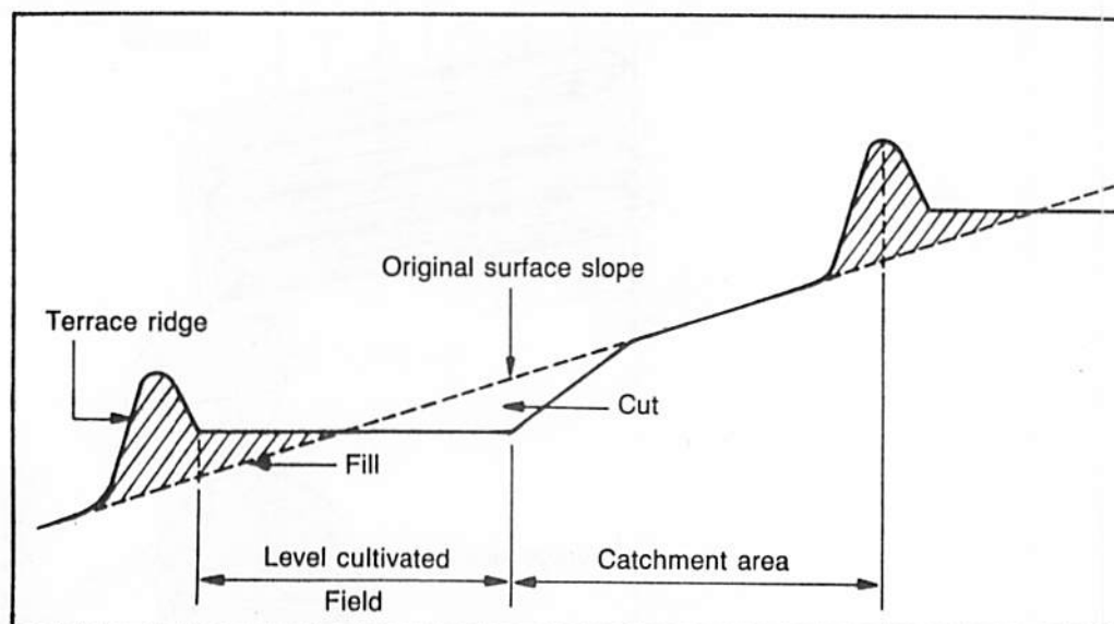
Figure 2. Diagram of Water Harvesting System with Catchment Area, Conveyance System, and Direct Application to Cultivated Field.
