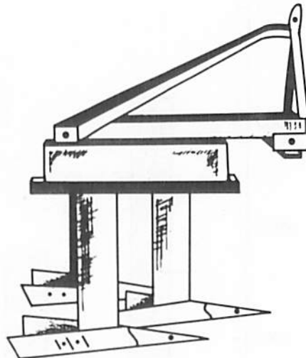
Figure 7. Large Sweep Which Is Used as the Initial Tillage Implement and for Succeeding Tillages (Dogan et al. , 1977).
