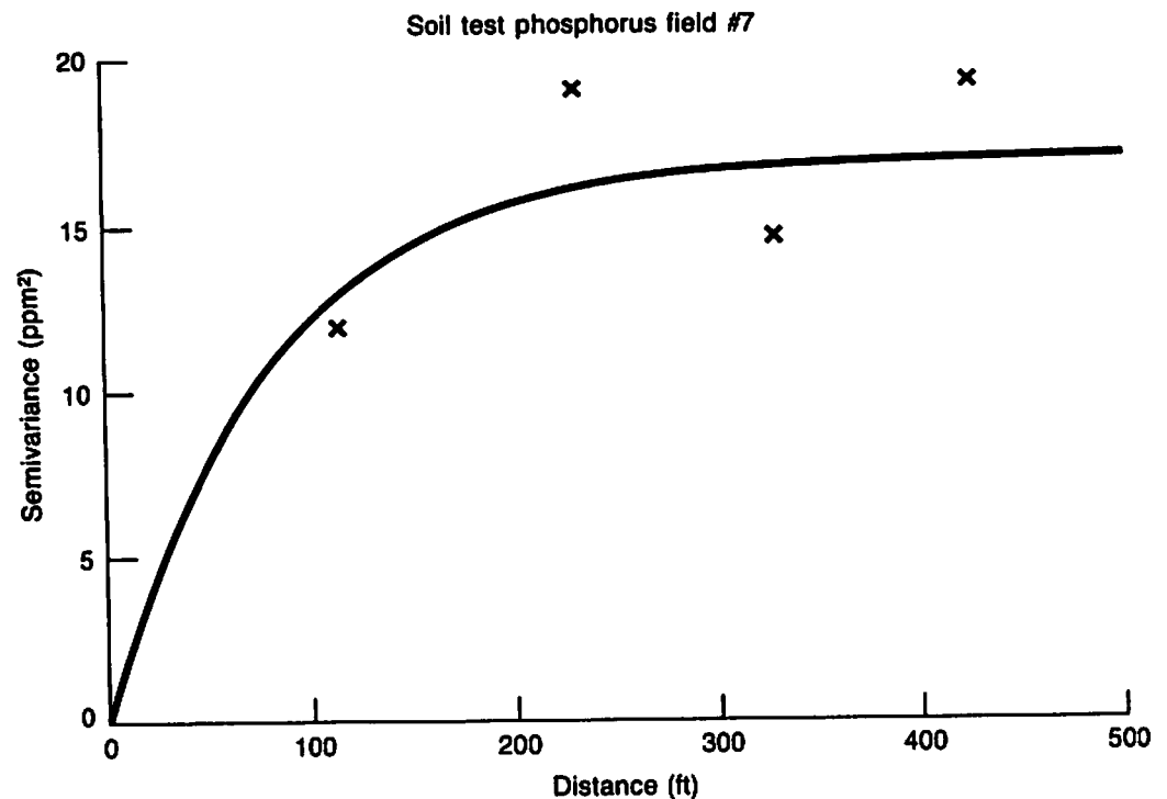
Figure 10. Semivariance Values and Exponential Semivariogram Model for 20 Soil Test Phosphorus Values on a Commercial Farm in the Columbia Basin of Washington.
