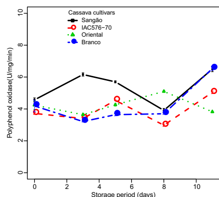
Figure 2. Changes in the activity of polyphenol oxidase in cassava cultivars during PPD. Each data point is presented as mean \pm standard deviation ( n = 3 ) in units per milligram*minutes ( \text{U mg}^{-1} \text{min}^{-1} ).
