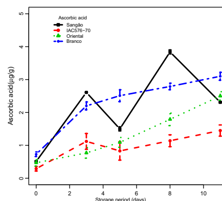
Figure 3. Changes in the concentrations of ascorbic acid in root samples of cassava cultivars during PPD. Each data point is presented as mean \pm standard deviation ( n = 3 ) in ( \mu\text{g g}^{-1} ).
