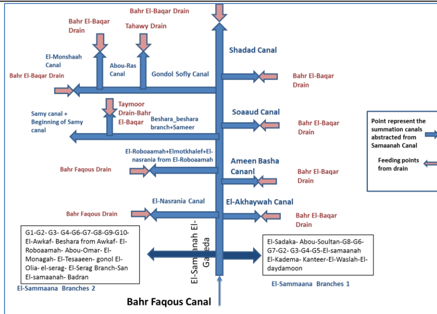
Figure 30: General Layout of Samaanah Canal
