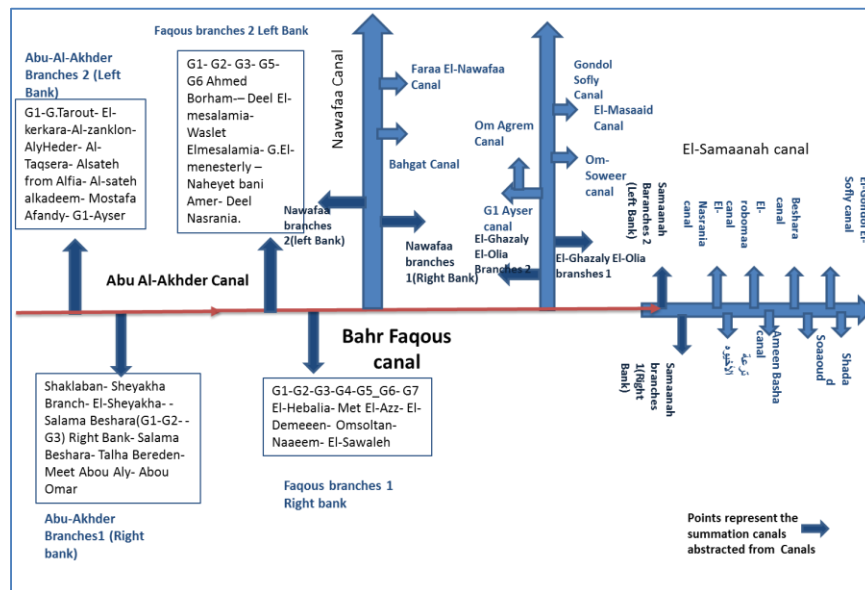
Figure 29: General Layout of modeled Irrigation System
