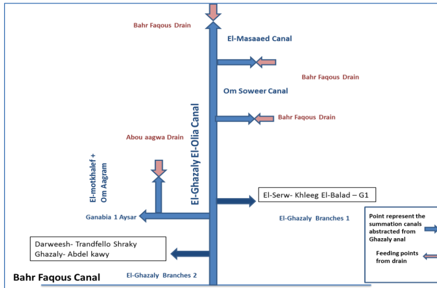
Figure 31: General Layout of Ghazaly Canal
